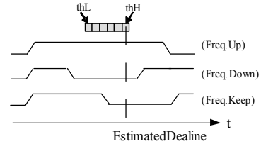
Figure 6. Adaptive frequency scheduling.
